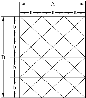
图2 矩形风口测点布置
