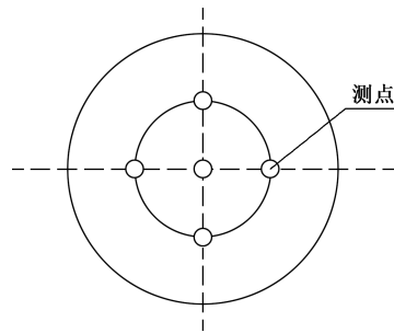
图4 圆形风口测点布置
